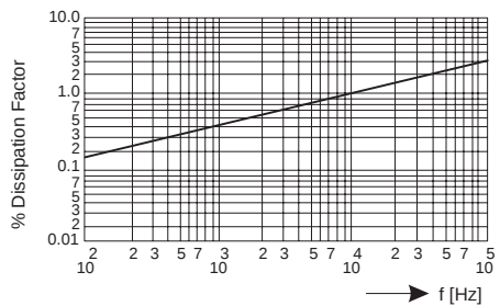
Dissipation Factor vs. Frequency (Room Temp.)
