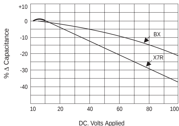
\Delta C vs. Voltage Coefficient
