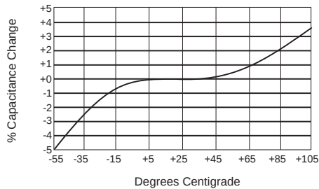
Capacitance Change vs. Temperature At 1KHz
