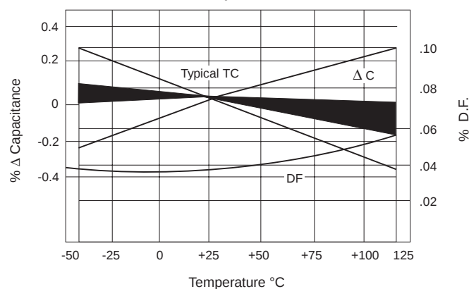
\Delta C , D.F. vs. Temperature Coefficient
