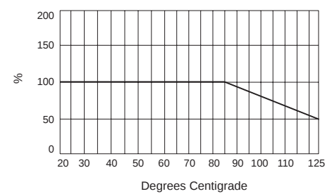
Voltage Derating vs. Temperature
