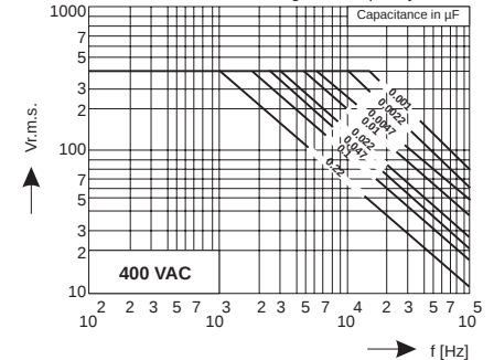
Permissible AC Voltage vs. Frequency
