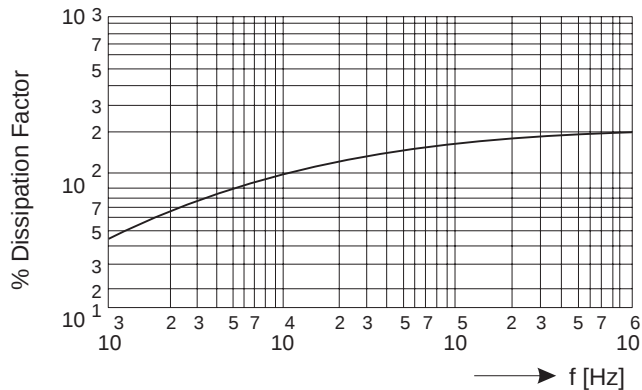
Dissipation Factor vs. Frequency (Room Temp.)
