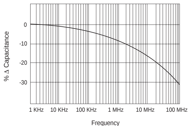
\Delta C vs. Frequency Coefficient
