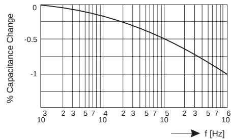
Capacitance Change vs. Frequency (Room Temp.)
