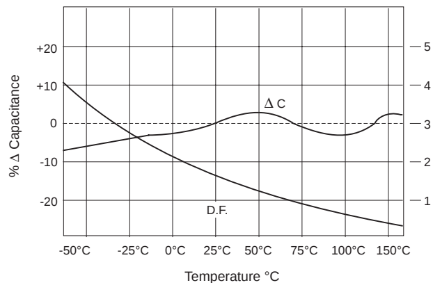
\Delta C, D.F. vs. Temperature Coefficient
