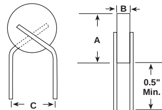
DIMENSIONAL CONFIGURATIONS
